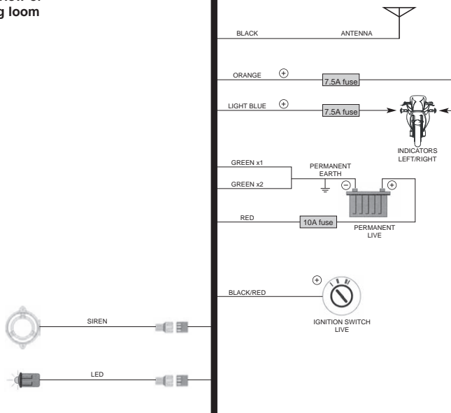
Rear view of wiring loom
