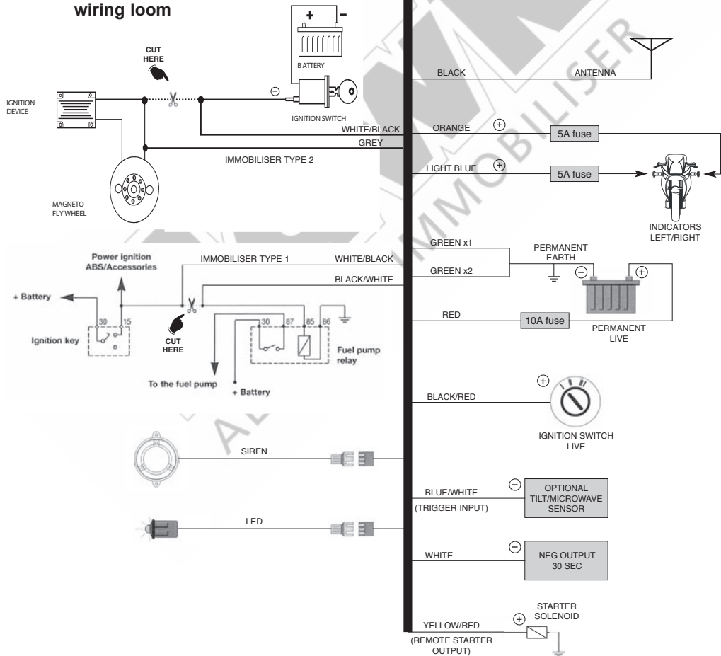
Rear view of wiring loom
